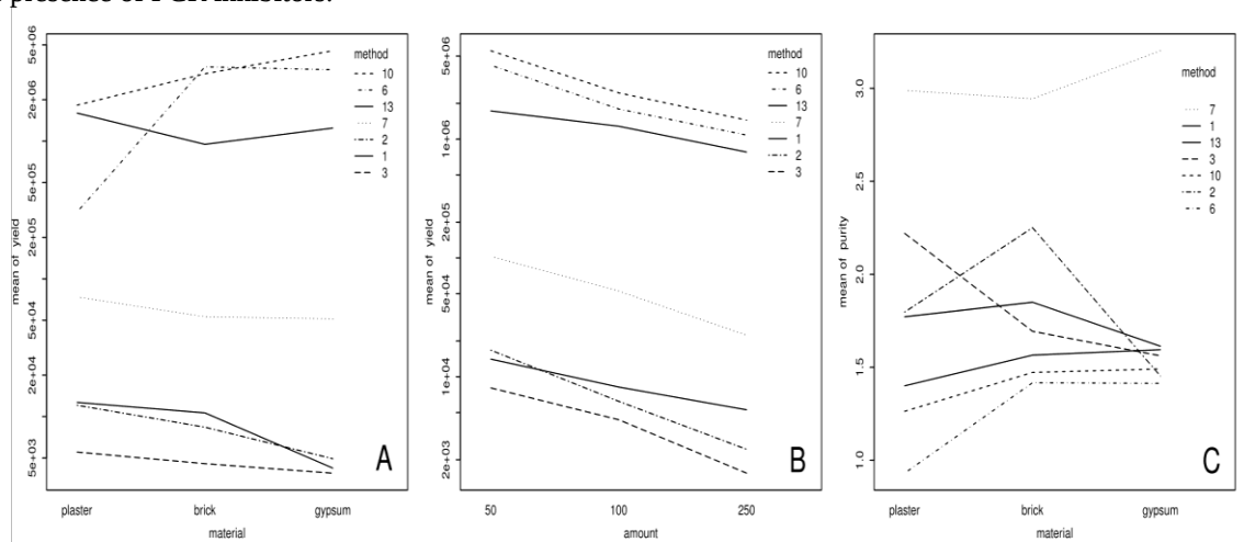
Fig. 2. Interaction plots of the mean values for measurement variables yield and purity of corresponding factor combinations are displayed and linked by profile lines for each method. (a) Mean values for yield of the factor combination material and method; (b) Mean values for yield of the factor combination sample amount and method; (c) Mean values for purity of the factor combination material and method.
